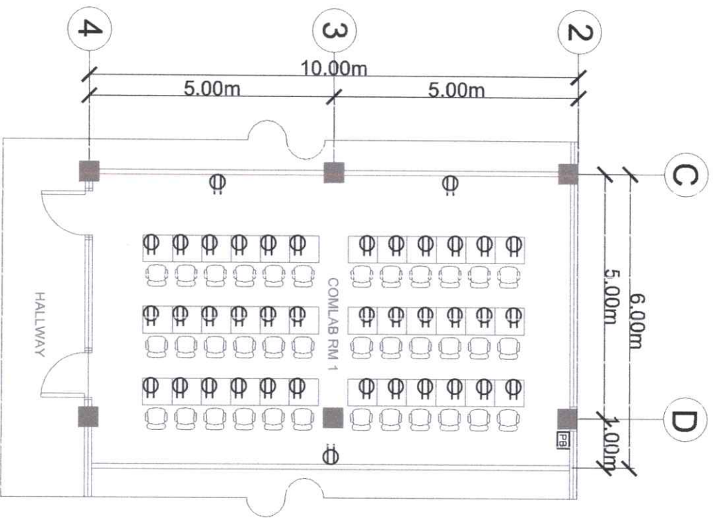
1 EXISTING COMLAB 1 POWER LAY-OUT E01 SCALE: 1:120M'S
