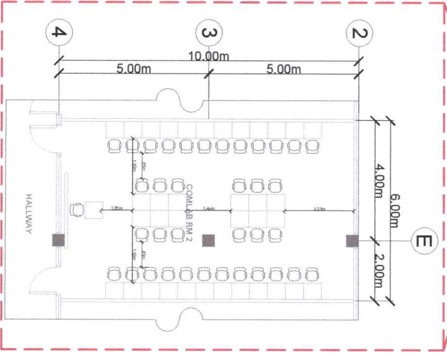
1 COMLAB 2 FLOOR PLAN 2ND FLOOR STGB BUILDING SCALE: 1:120MTS
