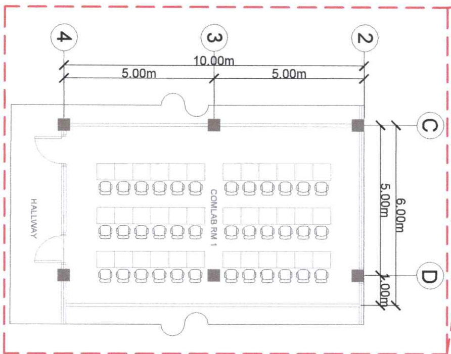
1 EXISTING FLOOR PLAN COM LAB 1, 2ND FLOOR STGB BUILDING A/01 SCALE: 1:120MTS
