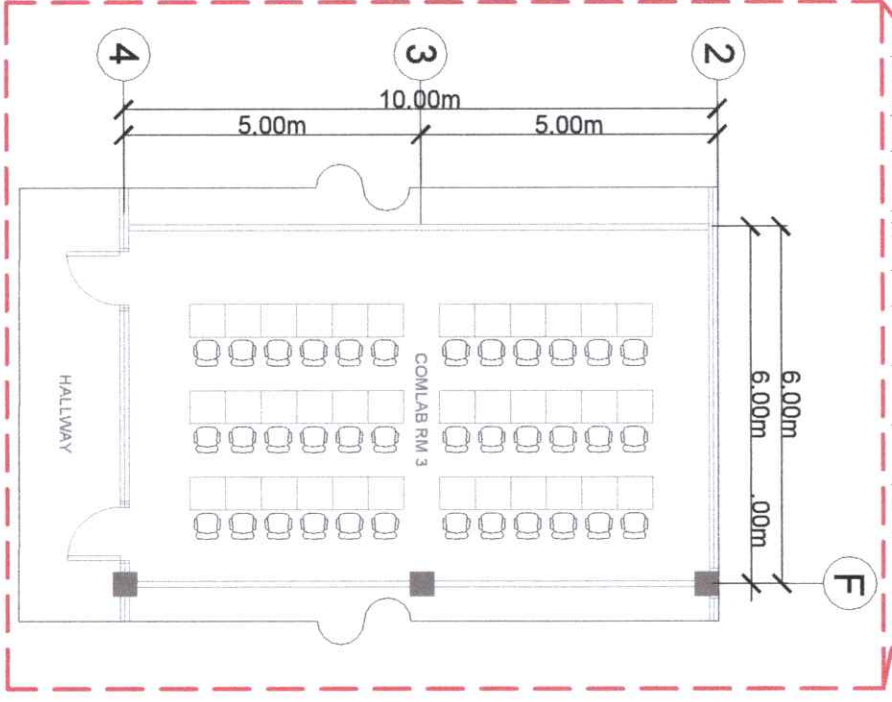
1 EXISTING FLOOR PLAN COM LAB 3, 2ND FLOOR STGB BUILDING A05 SCALE: 1:120MTS
