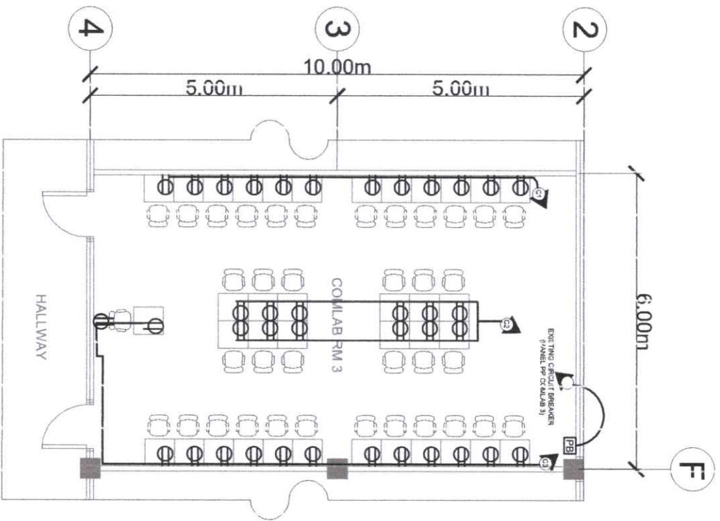
2 PROPOSED COMLAB 3 POWER LAY-OUT E03 SCALE: 1:120M/TS
