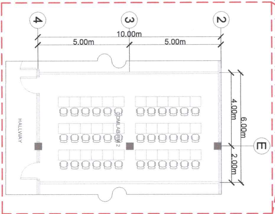
1 EXISTING FLOOR PLAN COM LAB 2, 2ND FLOOR STGB BUILDING A03 SCALE: 1:120MTS
