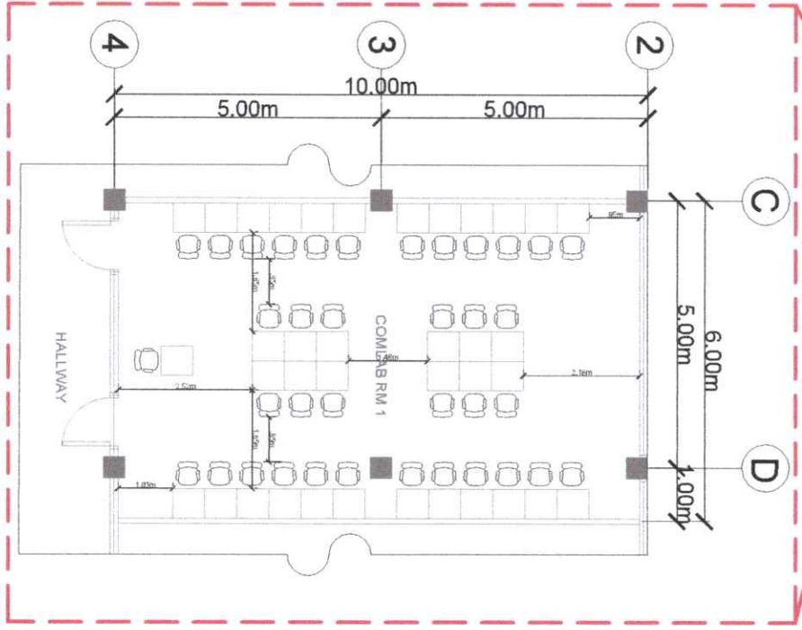
1 COMLAB 1 FLOOR PLAN 2ND FLOOR STGB BUILDING A02 SCALE: 1:120MTS
