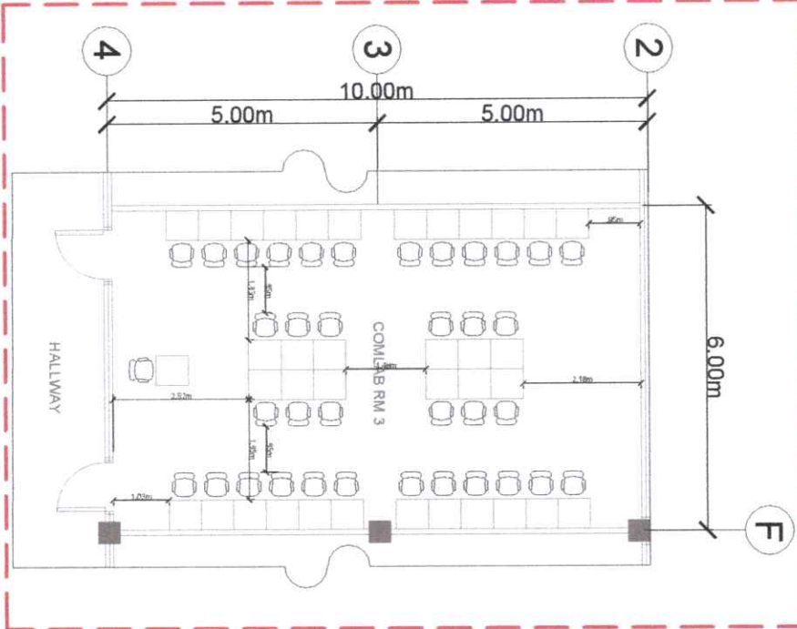
1 COMLAB 3 FLOOR PLAN 2ND FLOOR STGB BUILDING A06 SCALE: 1:120MTS
